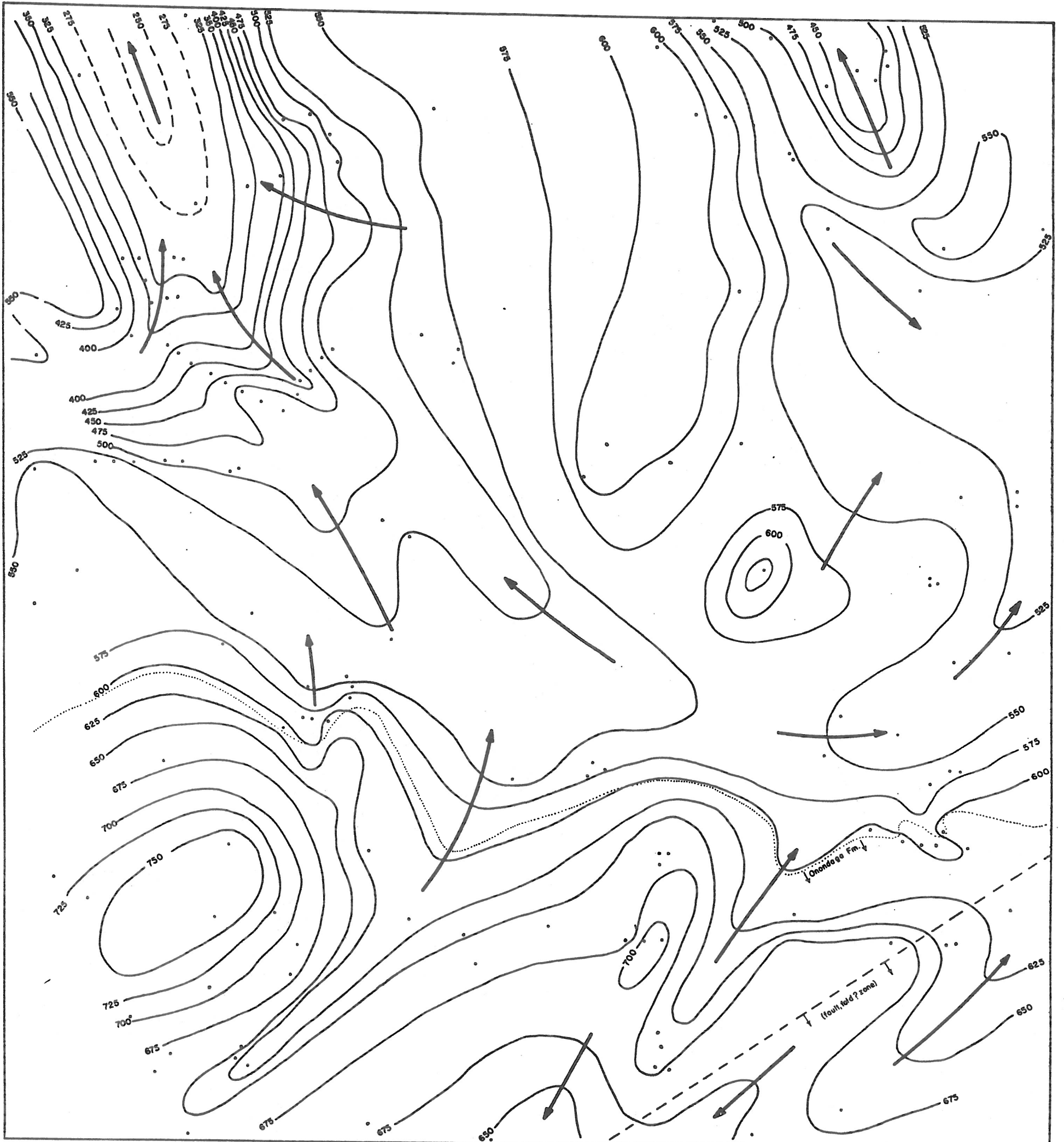
VICTOR, N.Y. APPROXIMATE BEDROCK SURFACE CONTOUR MAP.
